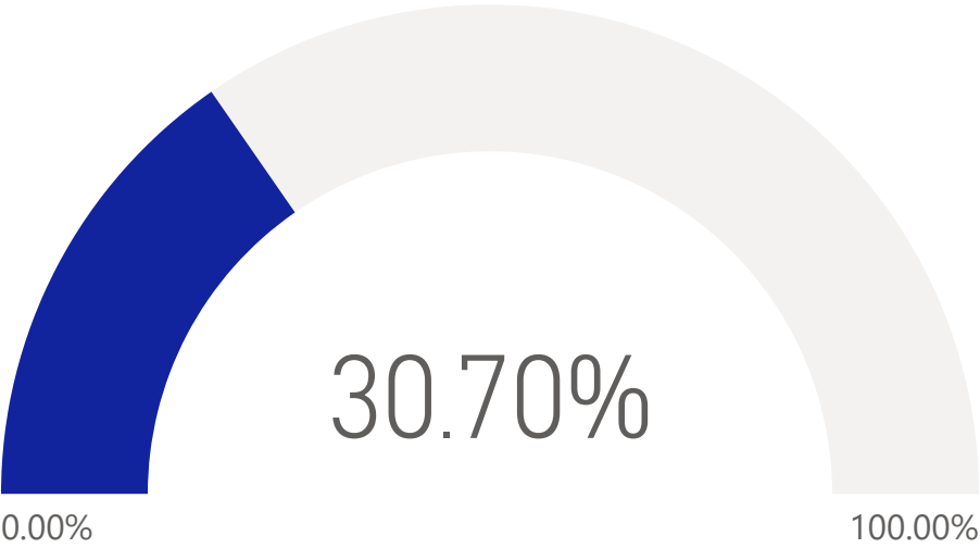
Bike Availability %
